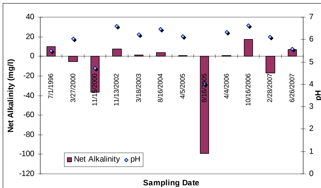
Figure 13. Net Alkalinity Levels at the Mouth of Brushy Creek (BC010), 2000-2006
