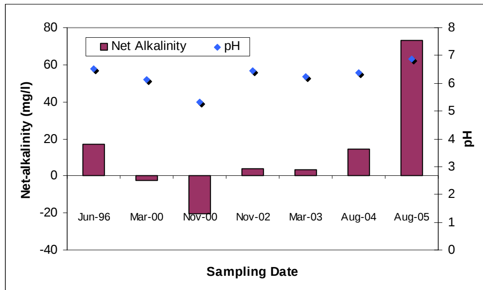
Figure 10. Net-Alkalinity and pH Data for the Mouth of West Branch (WB010)
