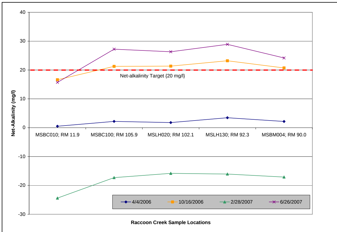
Figure 8. Net-Alkalinity Concentrations for Raccoon Creek Headwaters Mainstem Sites from 2006 - 2007
